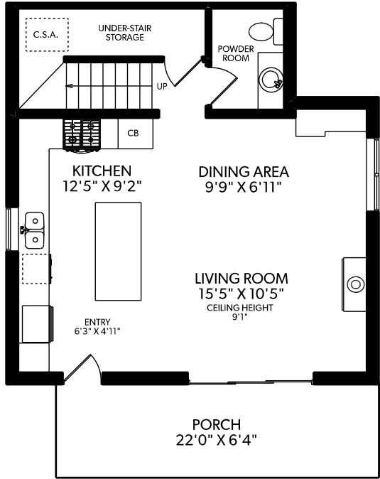
MAIN FLOOR
