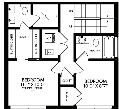
UPPER FLOOR
