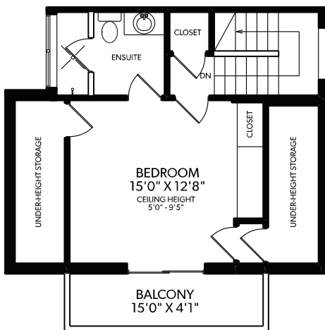
TOP FLOOR
