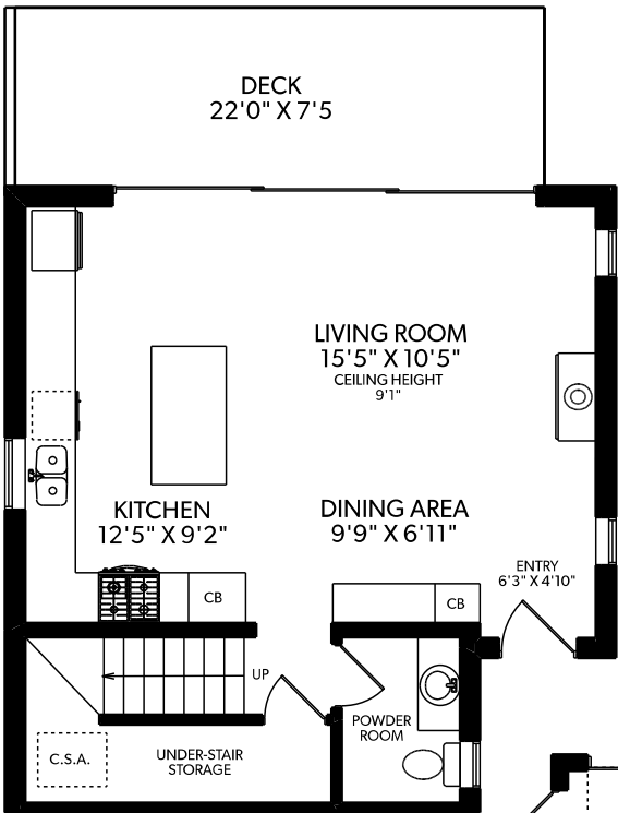
MAIN FLOOR
