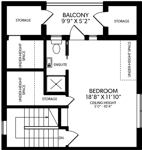
TOP FLOOR
