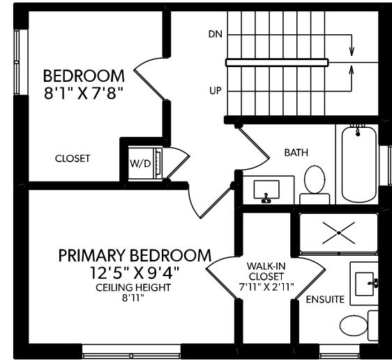
UPPER FLOOR
