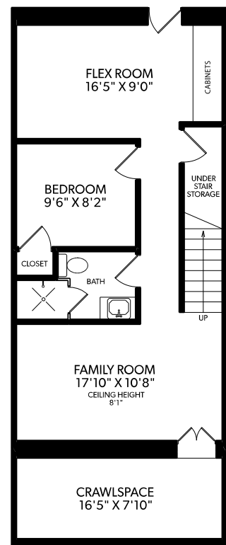
LOWER FLOOR
