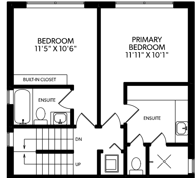
UPPER FLOOR
