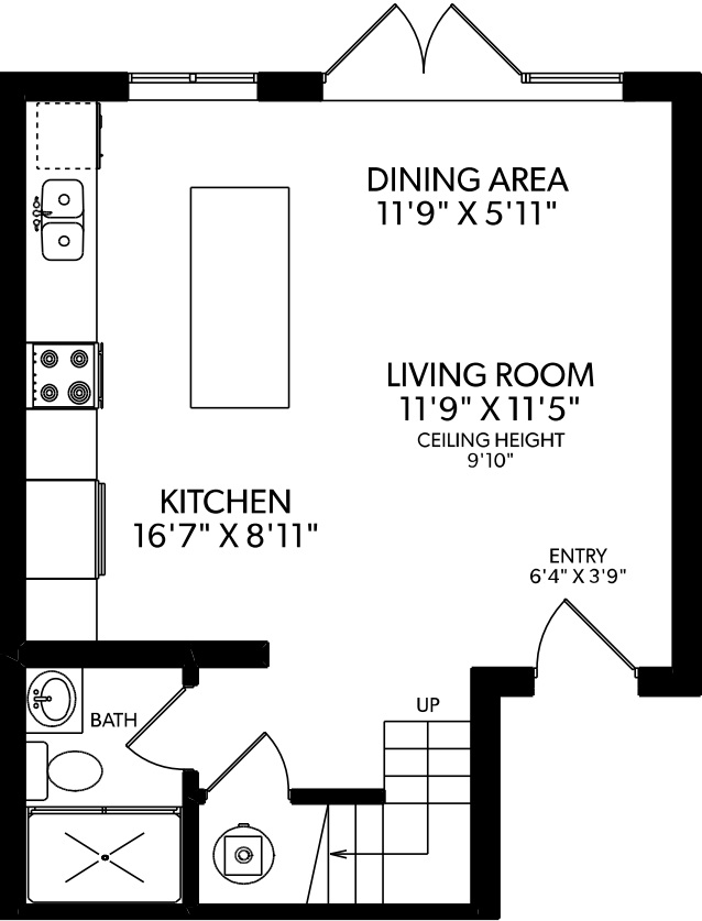
MAIN FLOOR
