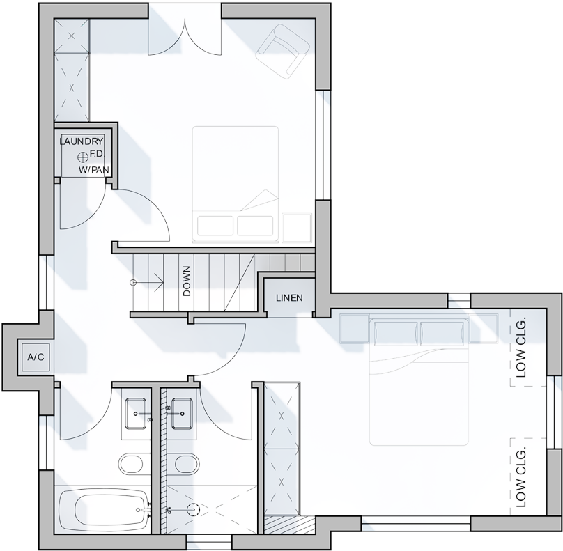
UPPER FLOOR
