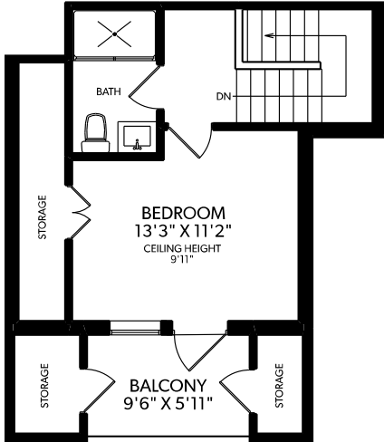
TOP FLOOR
