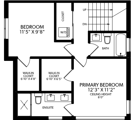
UPPER FLOOR
