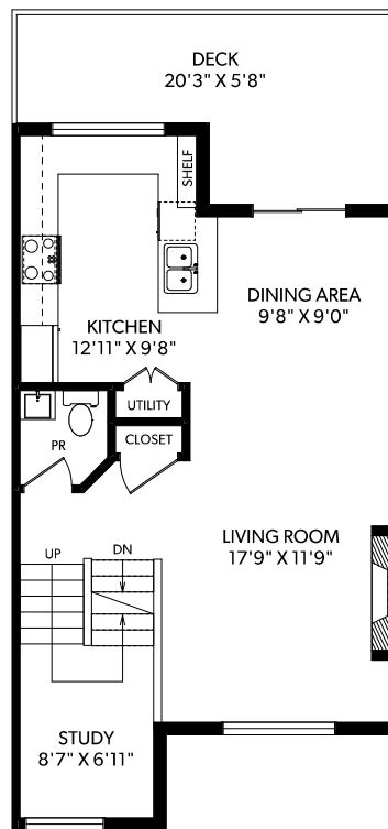
MAIN FLOOR
