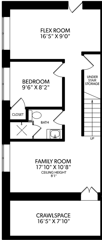
LOWER FLOOR
